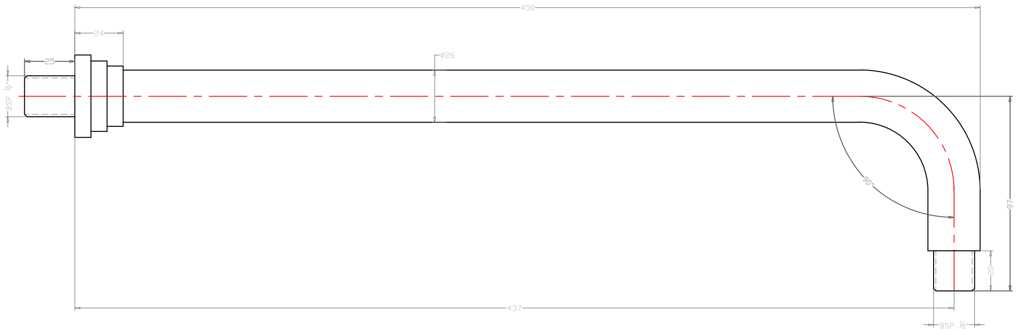
ADDONS-F160024 -HEAVY CASTED SHOWER ARM 450MM LONG WITH 90° BEND SUITABLE FOR RAIN SHOWER
